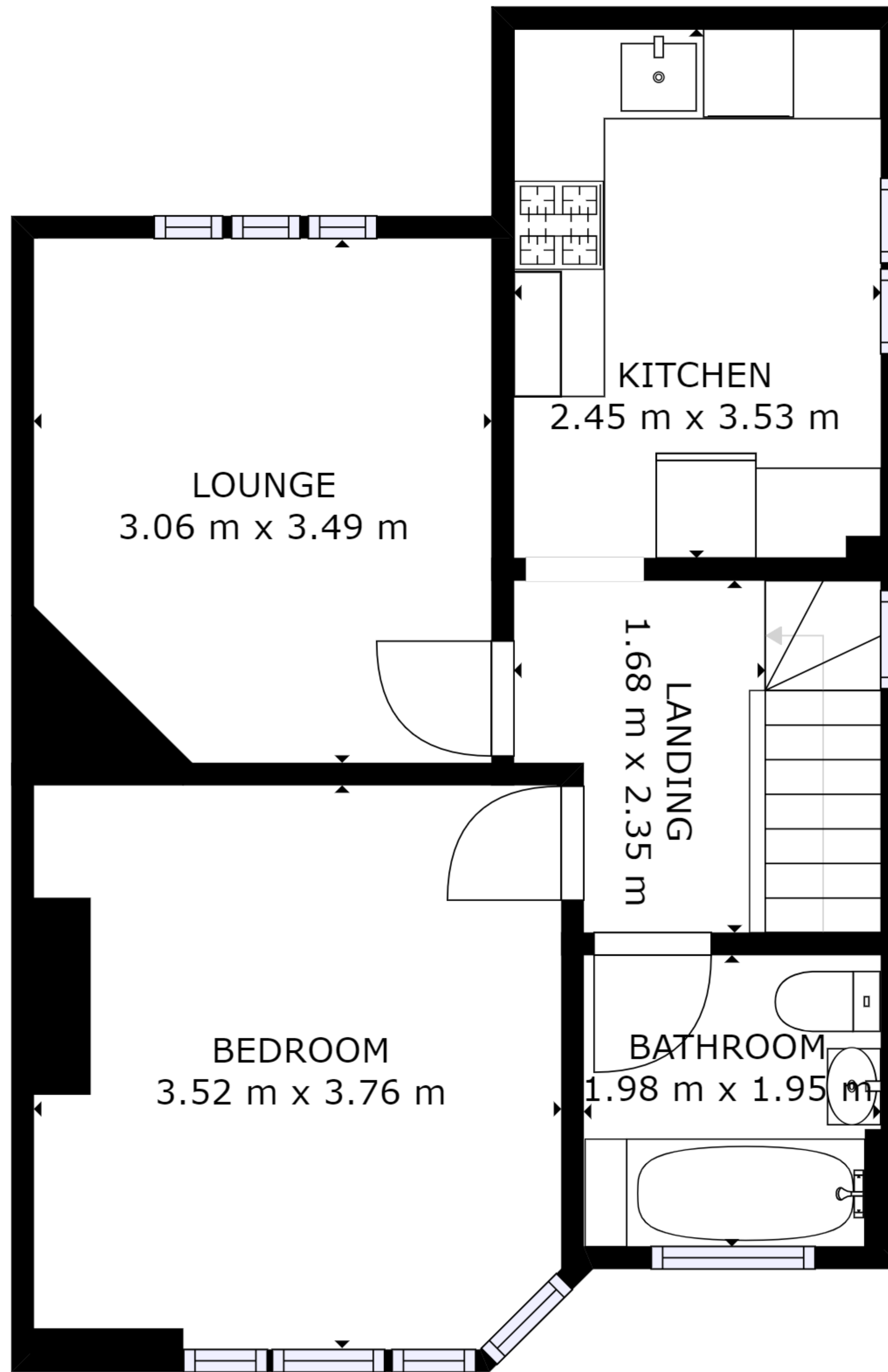
FLOOR 2
